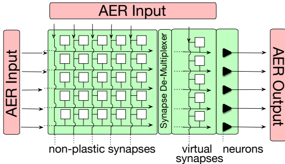
Fig. 1: Block-diagram of the ROLLS chip architecture.
