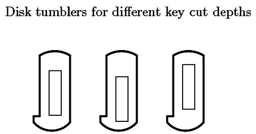
Figure 9.10: Working of a disk tumbler lock
