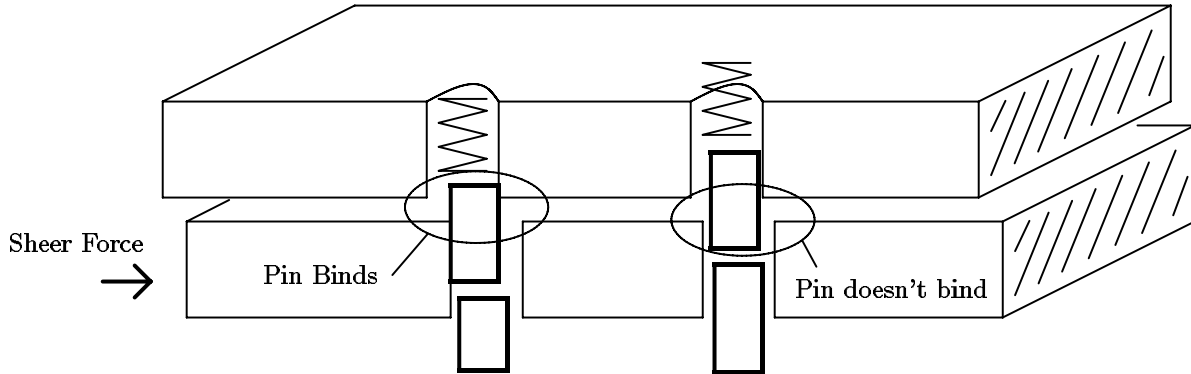
Figure 4.1: (a) Sheer force causes dri ver to bind
