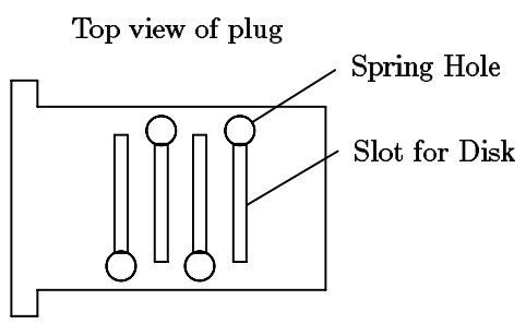
Figure 9.10: Working of a disk tumbler lock
