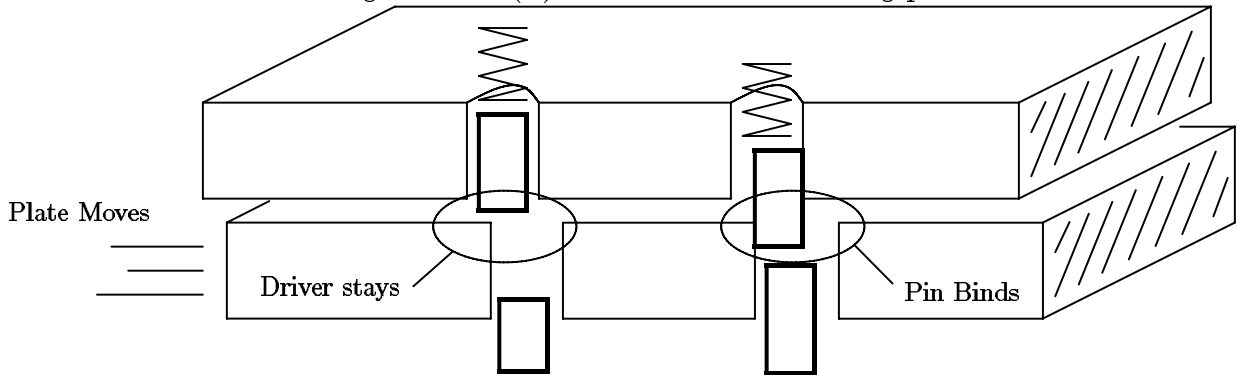
Figure 4.2: (b) Pi ck lifts the bi ndi ng pi n
