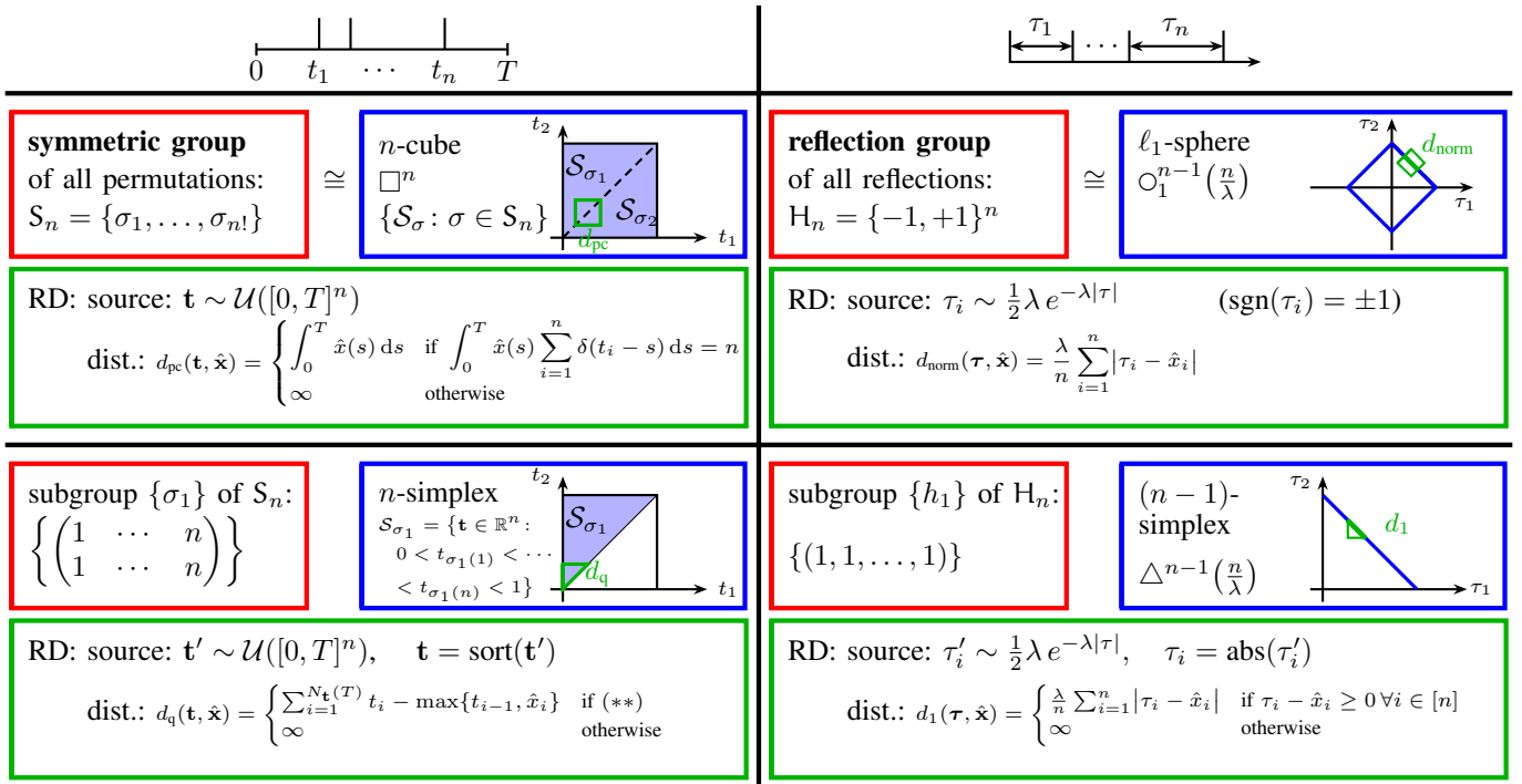
Fig. 1. Unification of four rate distortion problems. The left and right columns present the symmetries in the timing description (symmetric group) and the interval description (reflection group), respectively. The upper and lower rows present the respective group or its subgroup. Each quadrant also illustrates its own rate-distortion problem with its source set (in the blue box) and its natural distortion measure ‘dist’ (in the green box). In the left lower quadrant, we use Cauchy’s two-line notation for permutation to denote \sigma_1 ; and the (**) condition for finite distortion is N_{\hat{\mathbf{x}}}(T) = N_{\mathbf{t}}(T) and N_{\hat{\mathbf{x}}}(s) \geq N_{\mathbf{t}}(s) \forall s \in [0, T] . Note that the blue lines on the right column illustrate the region where the source is concentrated (when n \rightarrow \infty ).
