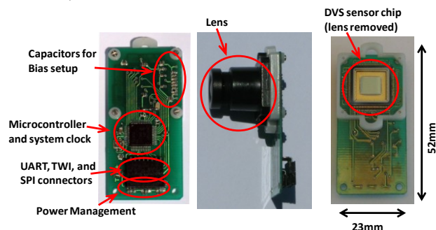
Figure 2: Embedded-DVS board showing functional elements.
