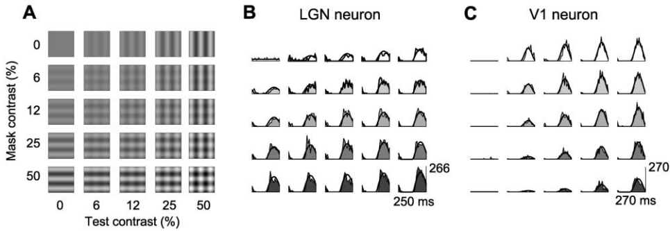
Figure 1. Cross-Orientation Suppression
